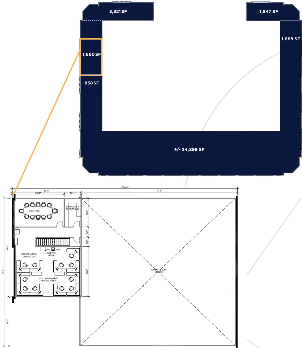
SECOND FLOOR Existing Plan, 4'x4' Design Grid
