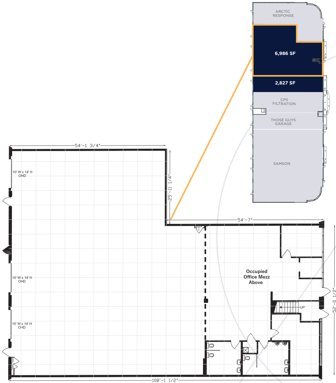
MAIN FLOOR Existing Plan, 5'x5' Design Grid
